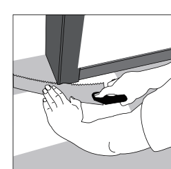
12 Door molding and skirting: lay a board (with the decorative side down) next to the door molding and as shown in the figure. Then slide the floorboard under molding.
