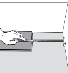
4 At the end of the first row, leave an expansion gap of 1/4" to the wall and measure the length of the last plank to fit.
