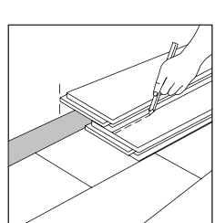
10 To lay the last row: position a loose board exactly on top of the last row laid. Place another board on top, with the tongue side touching the wall. Draw a line along the edge of this boards, to mark the first board. Cut along this line to obtain of the required width. Insert this cut board against the wall. The last row should be at least 2" wide. The spacers can then be removed.
