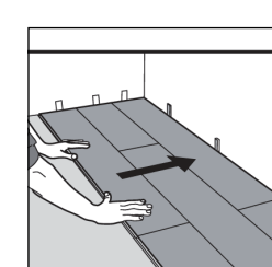
9 After 2-3 rows. Adjust the distance to the front wall by leaving an expansion gap of 1/4", always ensure that the end joints are staggered at least 8", both when in the same row as when from one row to the next one.
