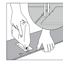
11 Holes for pipes: measure the diameter of the pipe and drill a hole that is 7/8" larger. Saw off a piece as shown in the figure and lay the board in place on the floor. Then lay the sawed-off piece in place.
