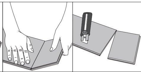
5 To cut the plank, use a simple utility knife and ruler, and with the top side facing up, cut heavily and several times on the same axis. The knife will not go through the surface but make a deep cut. You can then lift one half of the plank using your other hand to hold down the second placing it very close to the cut. The plank will split naturally.
