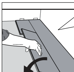
7 Click the long side of the plank into the previous row and place it tight to the short end of the previous plank with an angle of 30 degrees. Drop the plank and gently press down the end with a rubber mallet so it firmly locks into the previous plank until both are at the same height. Make sure both planks are perfectly aligned. NOTE: If you notice both planks aren't at the same height or are not well locked together, please follow the disassembling instructions at the bottom of the page, disassemble and check if any debris stuck inside the lock is obstructing.
